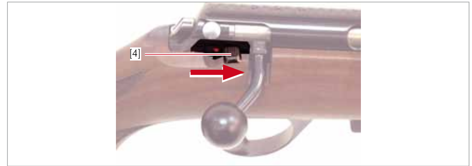
Fig.13 Sliding the safety catch forwards (releasing)
